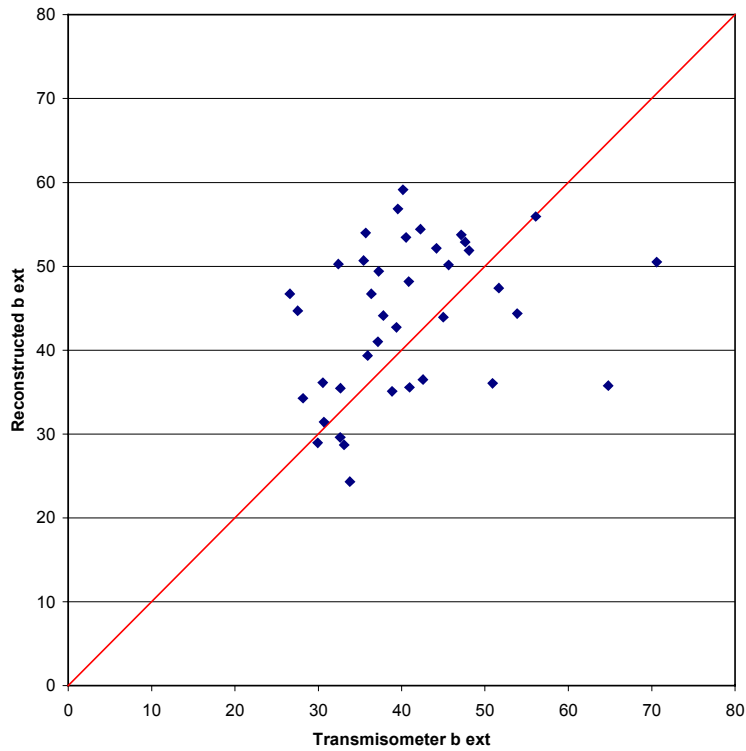
Figure 20: Comparison of measured extinction (transmissometer data) to reconstructed light extinction ( b_{ext} ; calculated using climatological mean monthly relative humidity adjustment factors) at Shenandoah National Park during 1999.
