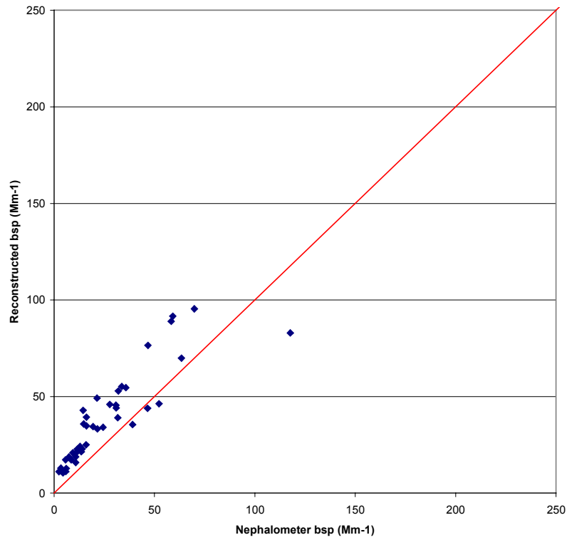
Figure 22: Comparison of measured scattering (nephelometer data) to reconstructed scattering ( b_{scat} ; calculated using daily relative humidity adjustment factors) at Acadia National Park during 1997.
