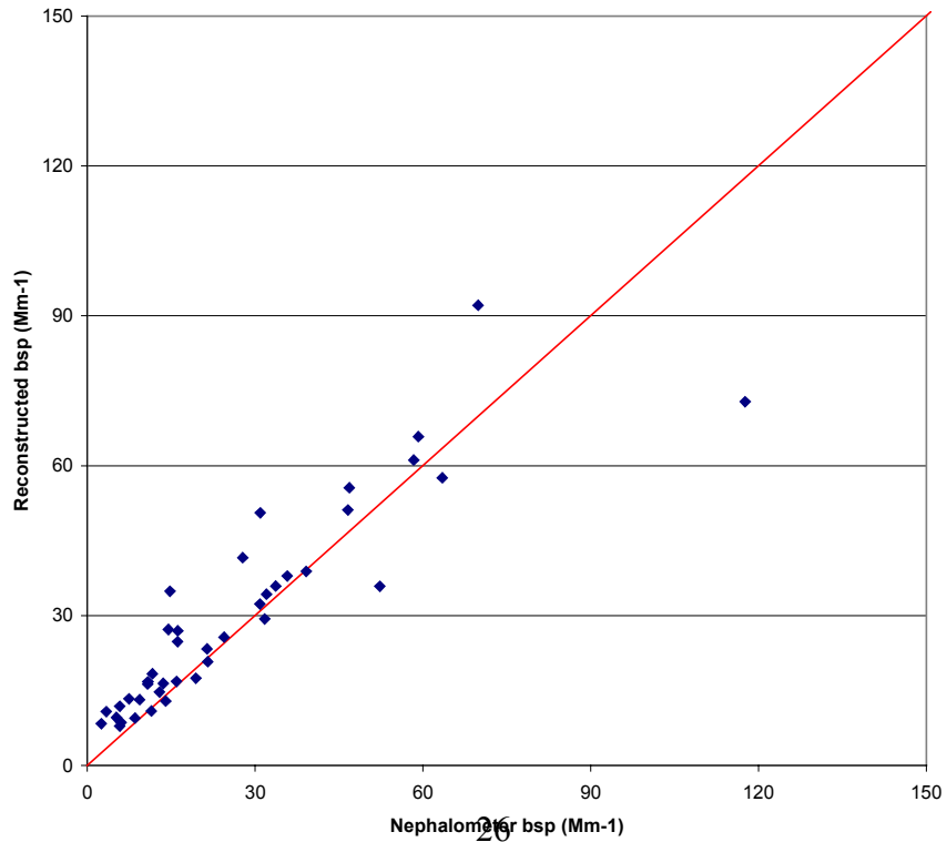
Figure 22: Comparison of measured scattering (nephelometer data) to reconstructed scattering ( b_{scat} ; calculated using daily relative humidity adjustment factors) at Acadia National Park during 1997.
