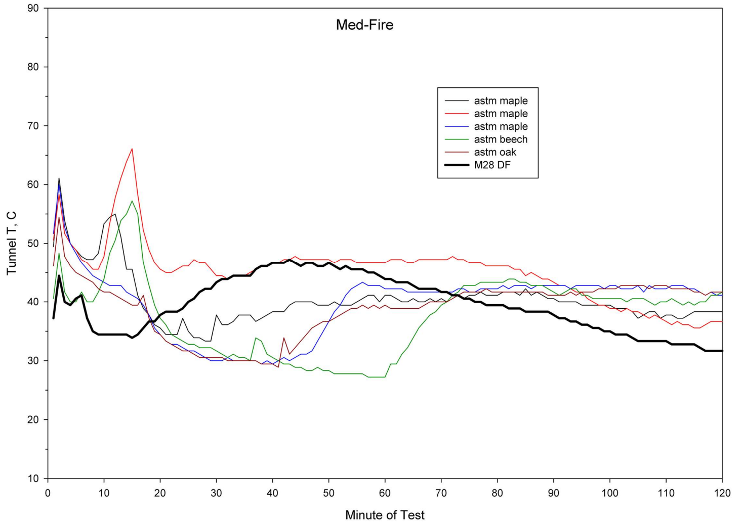
Figure A33-6. Comparison of Tunnel Temperatures ASTM @200 CFM: ASTM – Medium and M28 – Category 2/3
