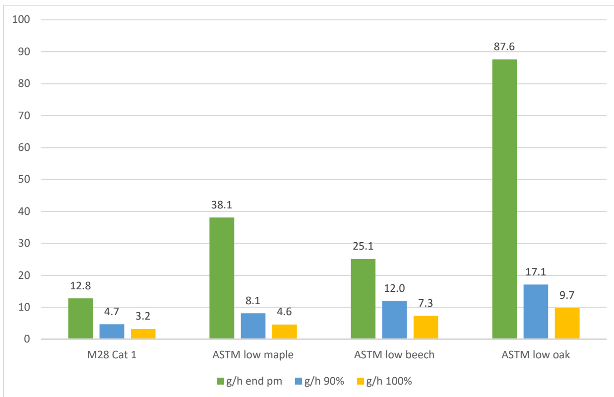
Figure A33-4. Comparison of PM Emission Rates (g/hr) at Medium Burn Rate
