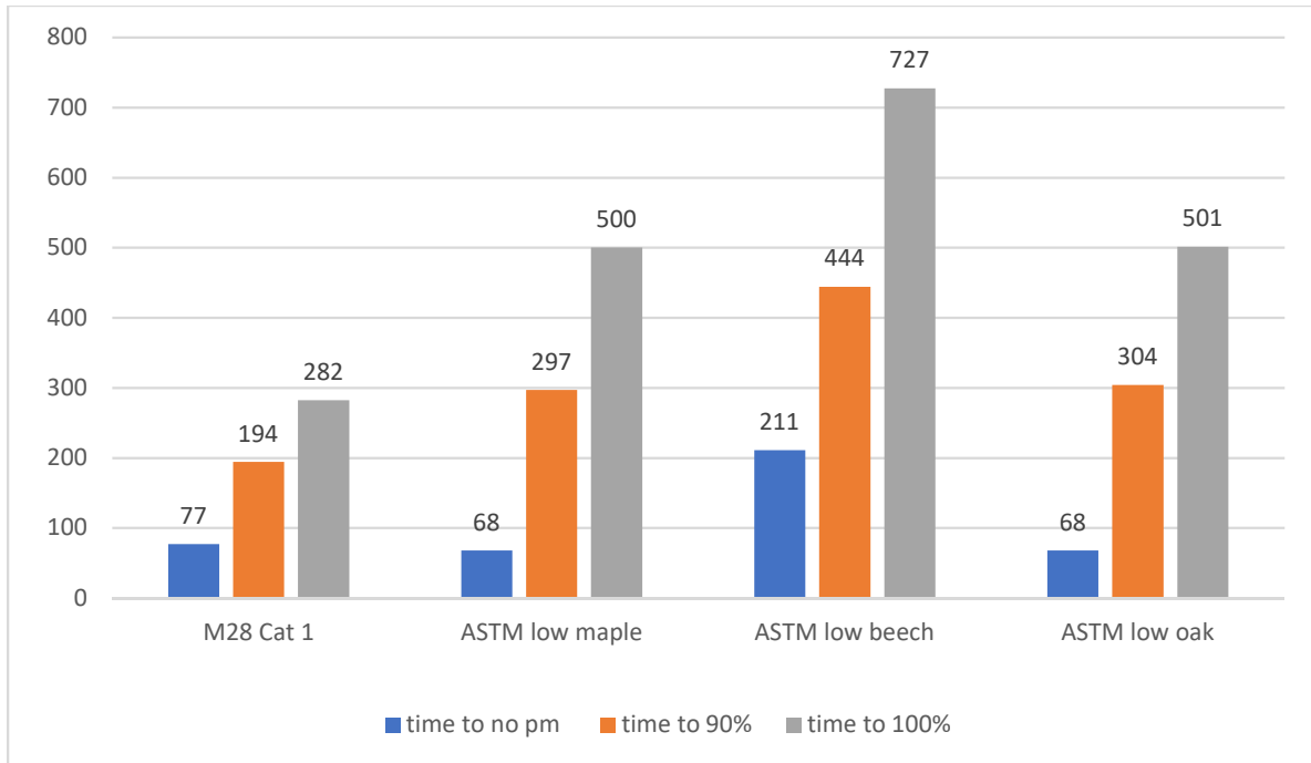
Figure A33-3. Comparison of Times (minutes) to for Key Events at Low Burn Rate
