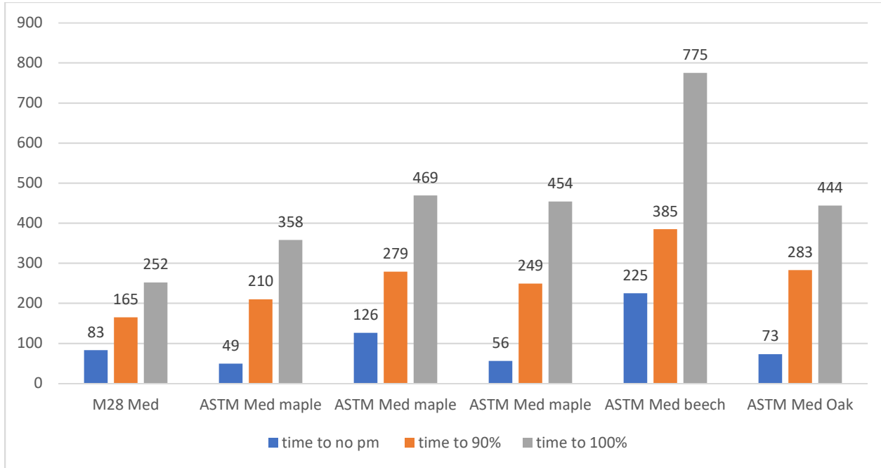
Figure A33-1. Comparison of Times (minutes) to for Key Events at Medium Burn Rate
