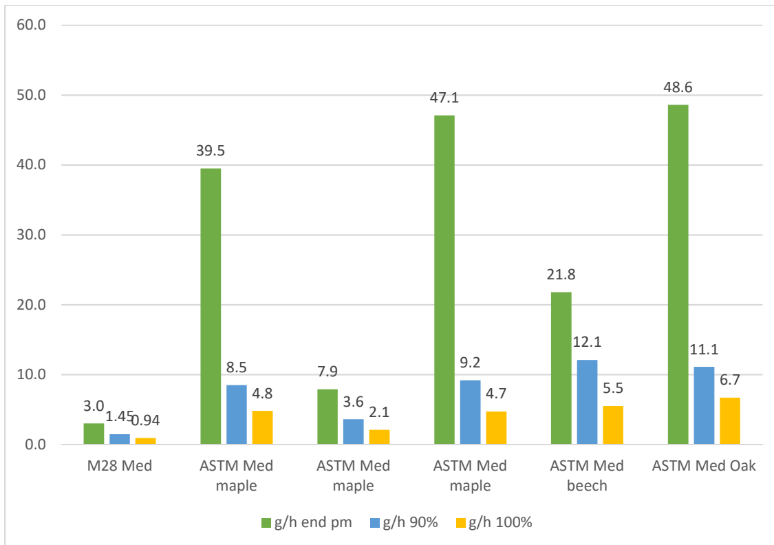
Figure A33-2. Comparison of PM Emission Rates (g/hr) at Medium Burn Rate
