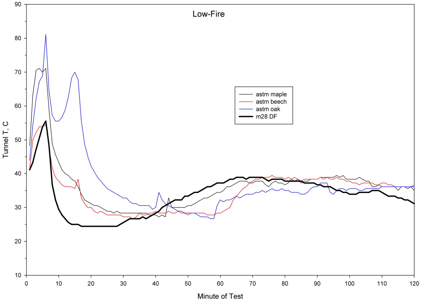
Figure A33-5. Comparison of Tunnel Temperatures ASTM @200 CFM: ASTM – Medium & M28 – Category 1
