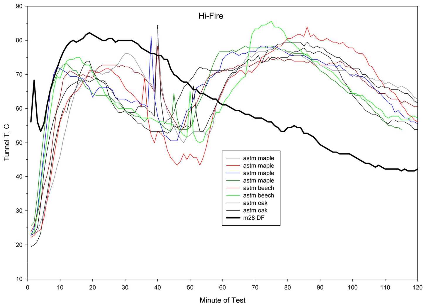
Figure A33-7. Comparison of Tunnel Temperatures @200 CFM: ASTM – High and M28 – Category 4
