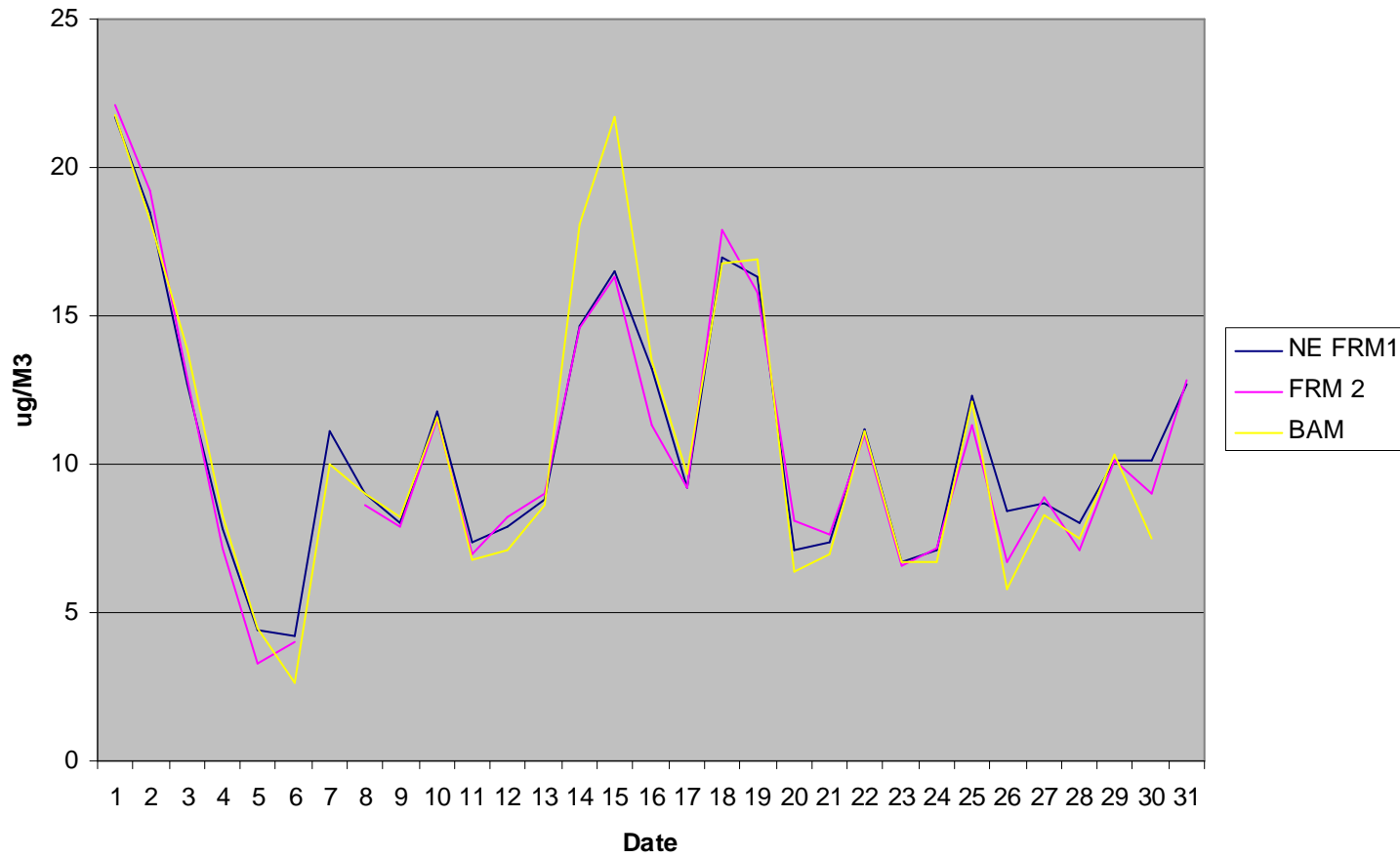
NEND BAM vs FRM August 2008
