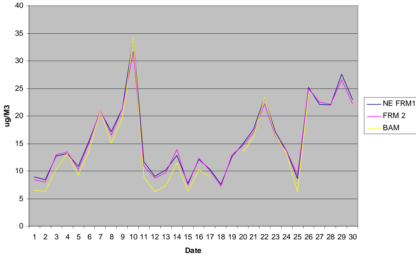
N End BAM vs FRM June 2008
