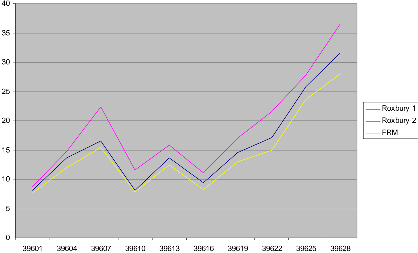
Rox BAMs vs FRM June 2008
