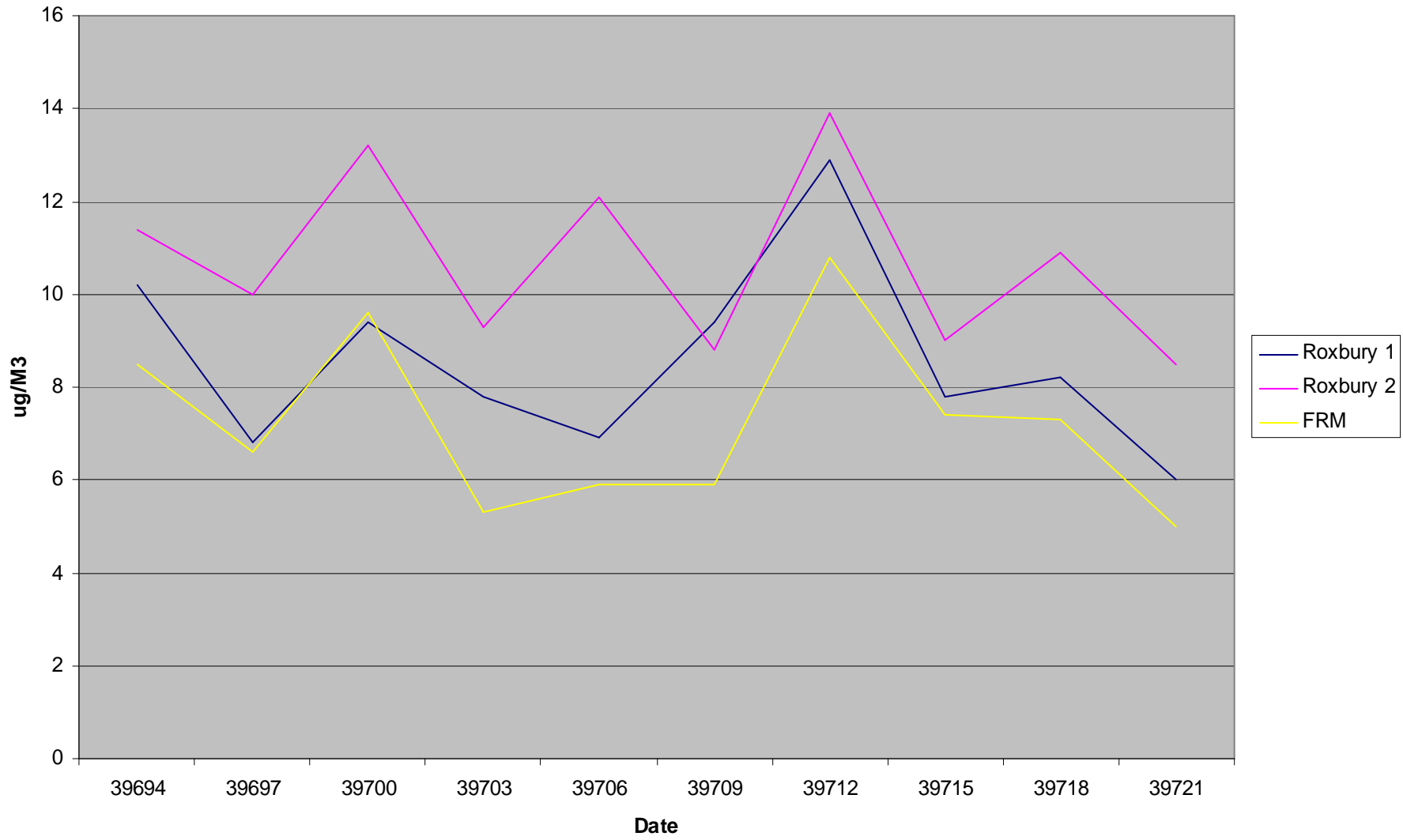
BAMs vs FRM Roxbury Sept 2008
