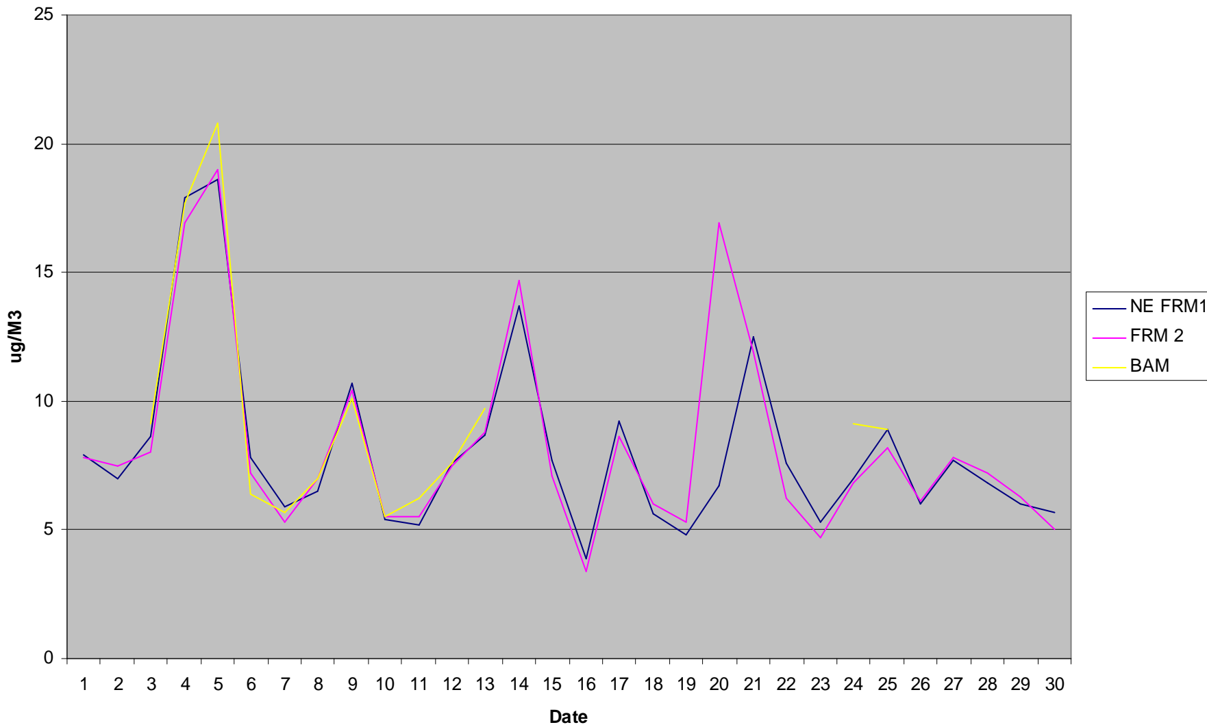
BAM vs North End FRM Sept 2008
